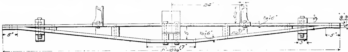
Fig. 1456. Elevation of Bolster.
